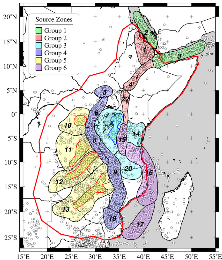
Fig. 2 Source zonation model used in this study (see Table 3 for details). Area sources belonging to same tectonic group are represented with unique colour. The outermost red solid line marks calculation area.
